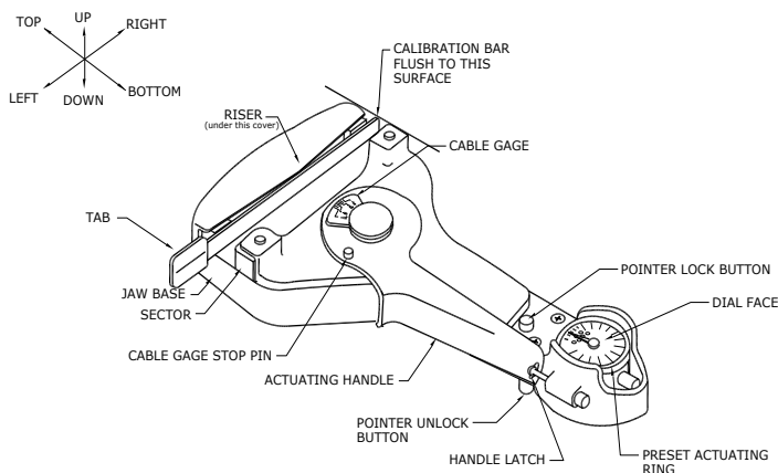
Figure 1 Cable Tensiometer, Typical
